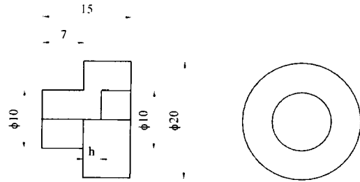
Fig. 8 Section view of hat-shaped specimen of SHPB shear test
