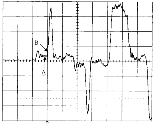
Fig. 9 A typical strain signal of transmit bar in shear test at impact velocity V=12.6 m/s ( h=0.5 , \delta=1.0 )
