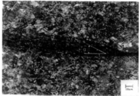
Fig. 12 Optical micrograph of tested hat-shaped specimen ( h=2 , \delta=0.5 , magnification : x50)
