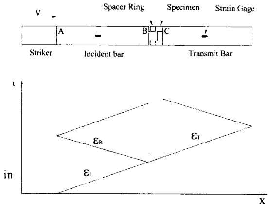
Fig. 1 The schematic of SHPB and characteristic diagram
