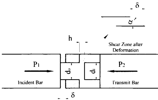
Fig. 2 Elastic bars and section view of the shear specimen
